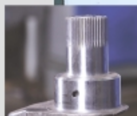
SERRATION ON GEAR END (DEEP ROLLING)
