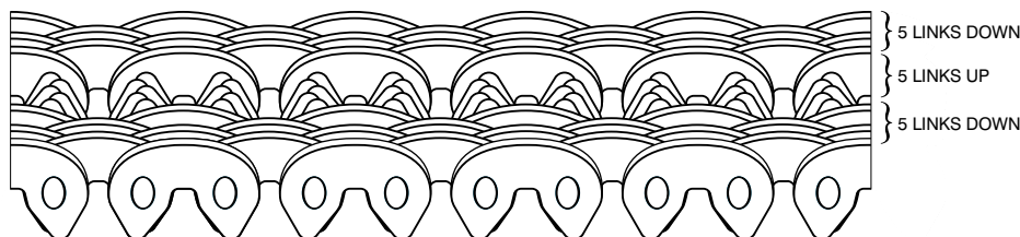
Typical Duplex Chain Assembly - RPDUP404 - 5-5-5 Assembly
