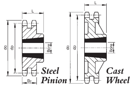
Duplex Sprockets Chain No. 10B-2
