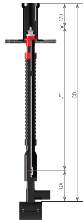
Definition of cover depth according to DVGW GW336
