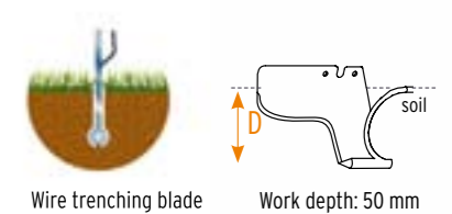
Wire trenching blade Work depth: 50 mm
