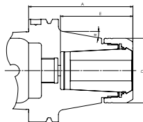
CENTROIP – Tapered Version for HPC Clamping Nuts
