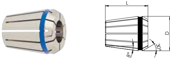
Precision Collets GERC-HP – 2 µm for GERC11-HP for GERC40-HP
