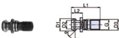
Pull Studs AZB ISO 7388-B without bore
