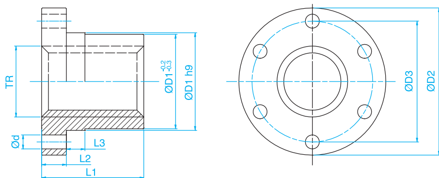
Colerette ronde Bronze CC493K (CuSn7ZnPb) selon ISO2901/2903 et DIN 103 tolérance 7H
