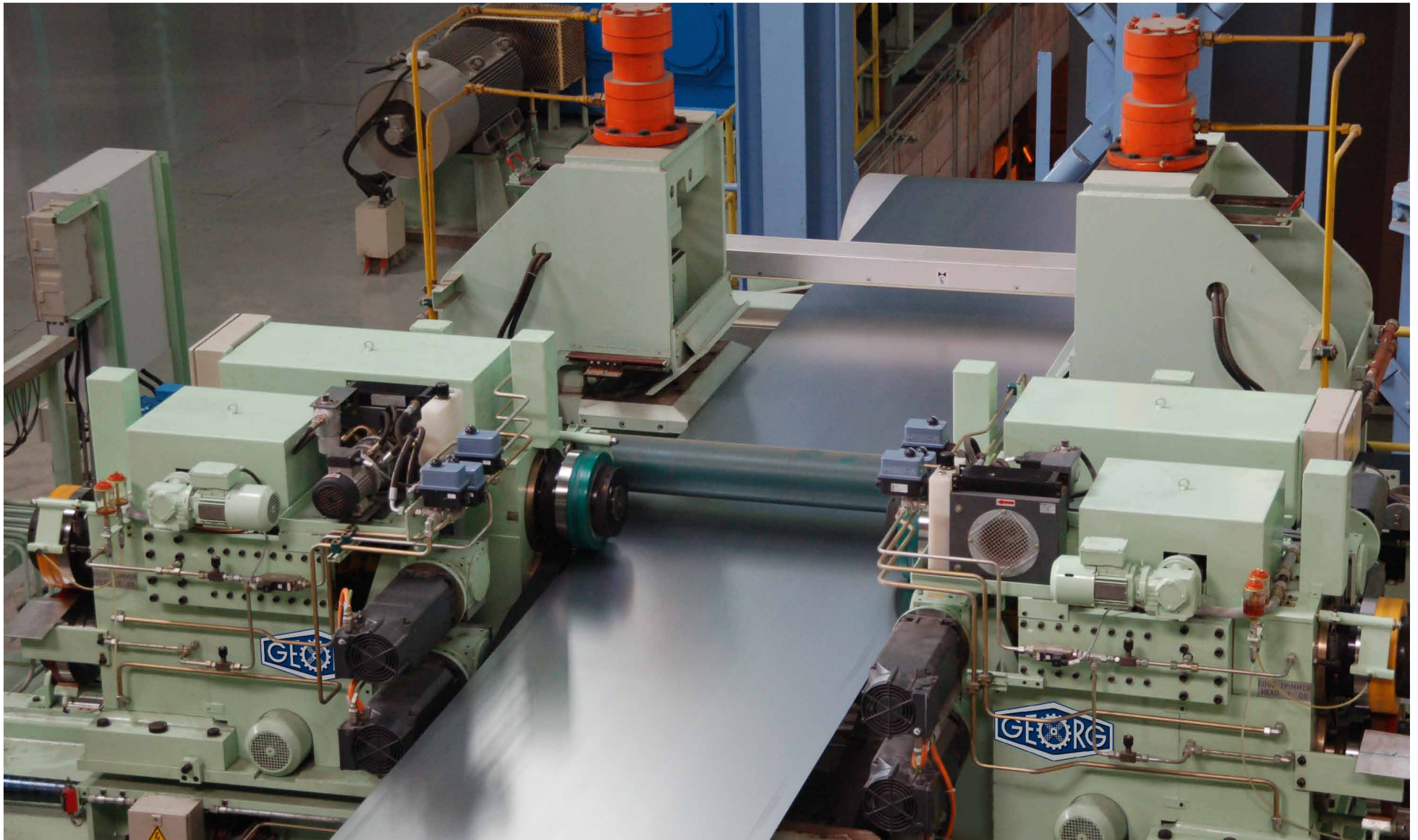
Turret type edge-trimming shear integrated in a galvanizing line
