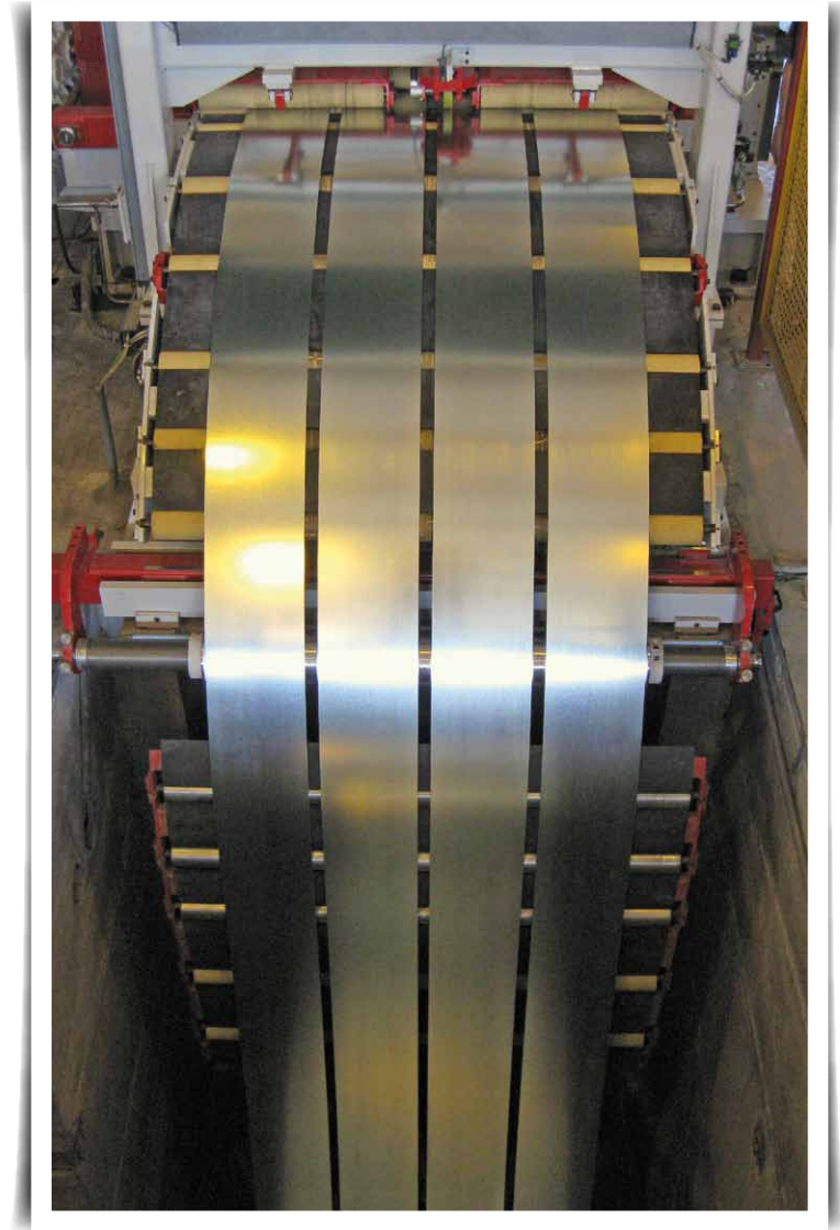
Exact guiding of the strands in the exit roller basket
