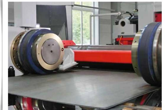
Edge-trimming shear for hot and cold rolled steel
