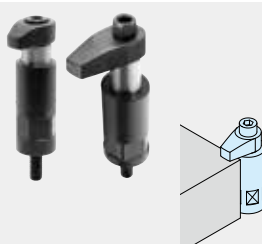
HOOK-CLAMP ASSEMBLIES
