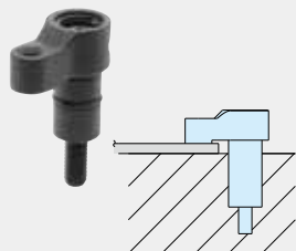
HOOK CLAMPS
