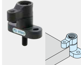
HOOK-CLAMP ASSEMBLIES WITH FLANGED HOLDER
