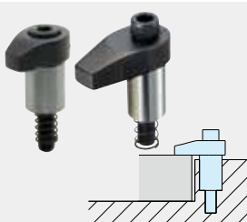
HOOK CLAMPS
