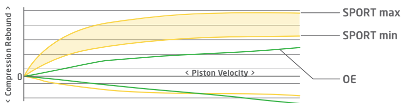
SPORT Damping Force Comparison
