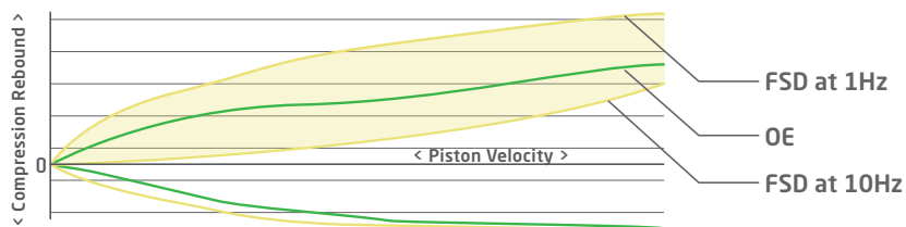
FSD Damping and Frequency Force Comparison
