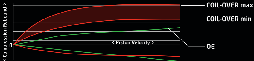
COIL-OVER Damping and Force Comparison
