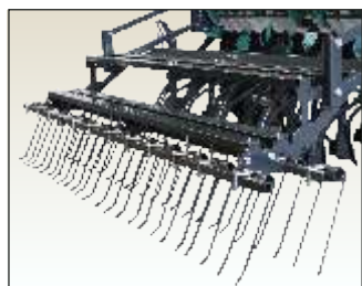
Erpice copriseme e pedana Seed covering harrow with foot board- Herse couvre-graines et passerelle Grada cubresemilla y plataforma
