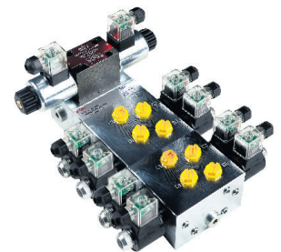
4 block LS
