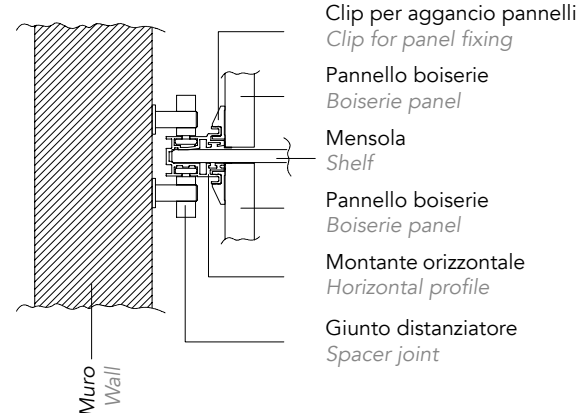
DETAIL 2 a) Aggancio a muro Wall mounting
