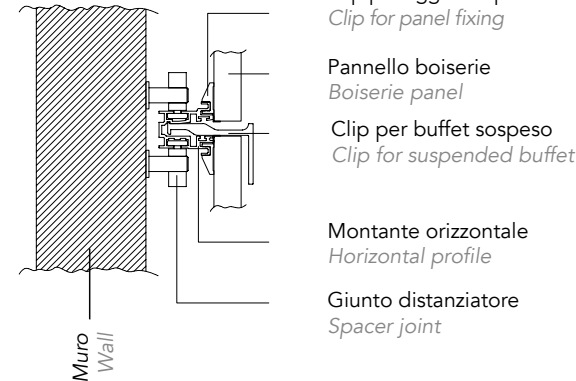
DETAIL 3 a) Aggancio a muro Wall mounting
