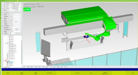
Off-line programming
