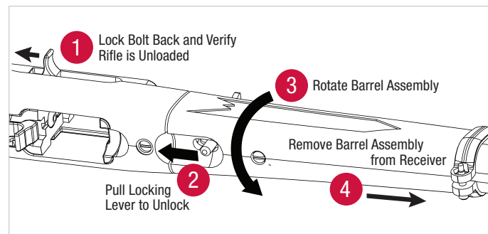
Takedown Enables Quick and Easy Separation of the Barrel from the Action
