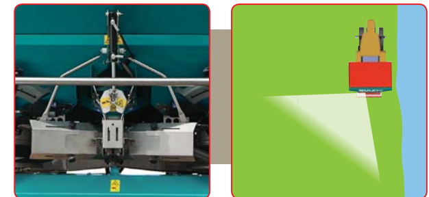
"Half-width" border spreading deflector with hydraulic control (1 DA) from the cab, left or right side
