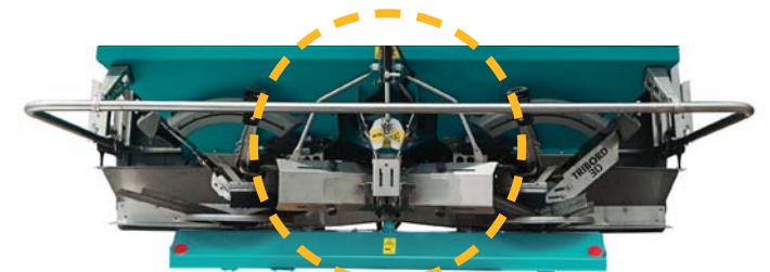
"Half-width" border spreading deflector with hydraulic control (1 DA) from the cab
