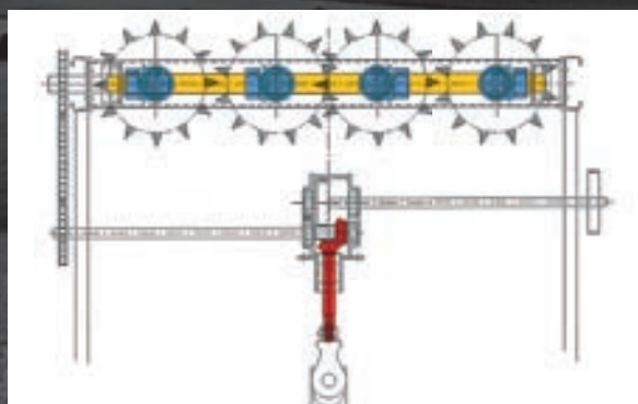
CS 70 - CS 80 - CS 90 Spreader device with reduction gear.
