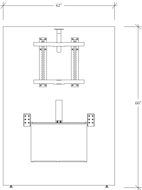
Without Tek Shelf
