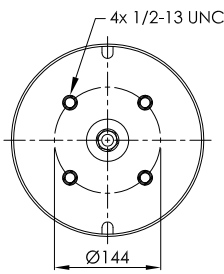
STEEL PISTON
