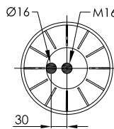
PLASTIC PISTON
