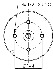
STEEL PISTON
