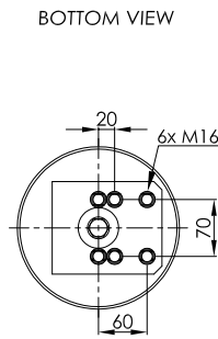
PLASTIC PISTON
