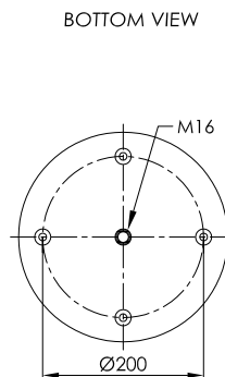
STEEL PISTON
