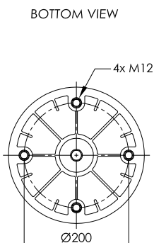
PLASTIC PISTON
