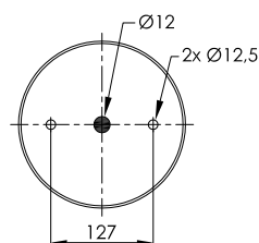
STEEL PISTON
