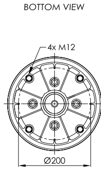
PLASTIC PISTON
