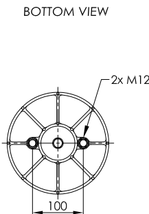
PLASTIC PISTON
