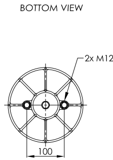
PLASTIC PISTON
