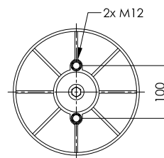
PLASTIC PISTON
