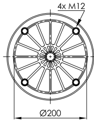
PLASTIC PISTON
