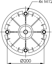
PLASTIC PISTON
