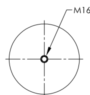
STEEL PISTON
