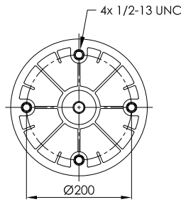
PLASTIC PISTON
