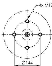
STEEL PISTON
