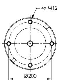
STEEL PISTON
