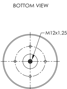
STEEL PISTON
