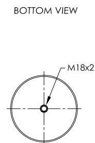
STEEL PISTON
