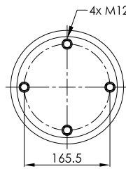
STEEL PISTON
