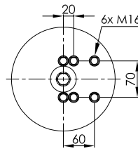
STEEL PISTON
