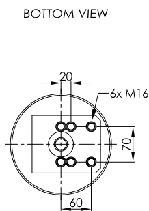
PLASTIC PISTON
