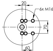
STEEL PISTON
