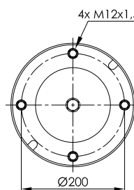
STEEL PISTON
