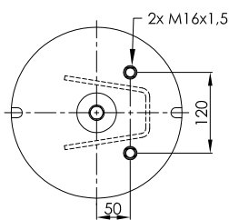
STEEL PISTON
