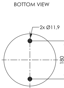
STEEL PISTON
