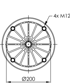
PLASTIC PISTON
