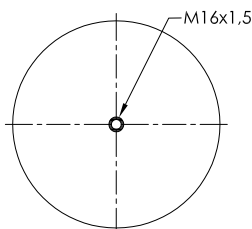
STEEL PISTON
