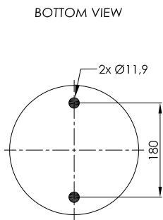
STEEL PISTON
