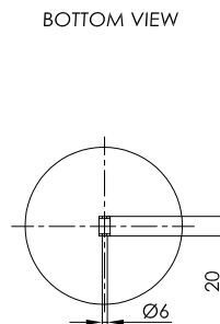
STEEL PISTON
