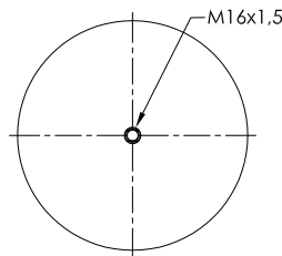
STEEL PISTON
