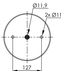
STEEL PISTON
