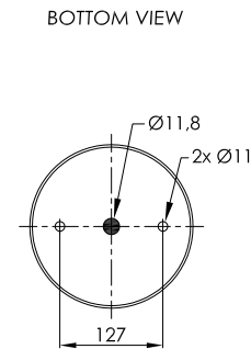
STEEL PISTON
