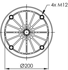
PLASTIC PISTON
