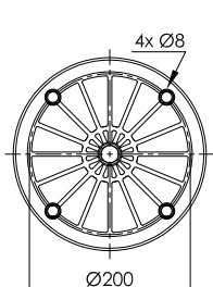
PLASTIC PISTON
