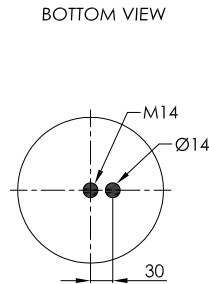
STEEL PISTON
