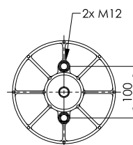
PLASTIC PISTON
