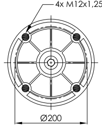
PLASTIC PISTON
