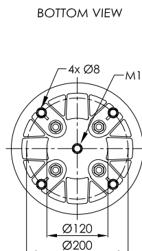
PLASTIC PISTON
