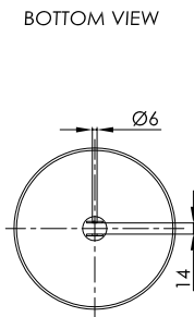
STEEL PISTON
