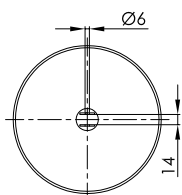
STEEL PISTON
