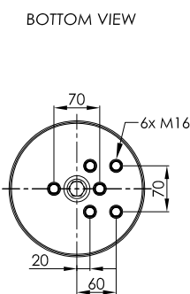
STEEL PISTON
