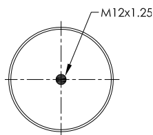
STEEL PISTON
