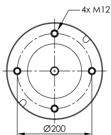
STEEL PISTON
