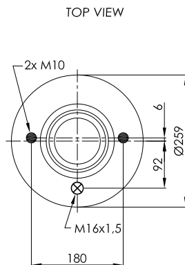
STEEL PISTON
