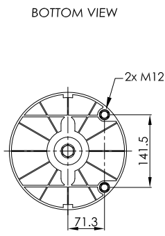
PLASTIC PISTON
