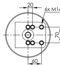
PLASTIC PISTON
