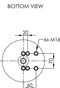
STEEL PISTON
