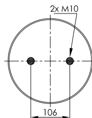
STEEL PISTON
