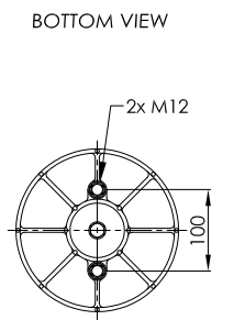
PLASTIC PISTON
