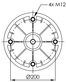
PLASTIC PISTON
