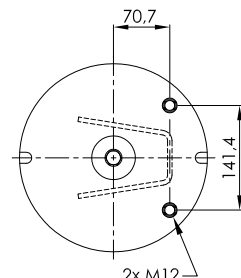
STEEL PISTON
