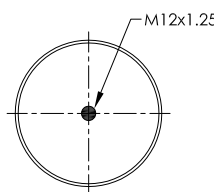
STEEL PISTON
