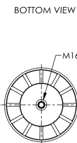
PLASTIC PISTON
