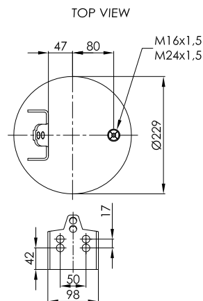
STEEL PISTON
