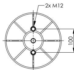
PLASTIC PISTON
