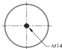
STEEL PISTON
