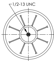
PLASTIC PISTON
