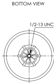
PLASTIC PISTON
