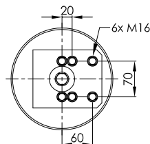
PLASTIC PISTON
