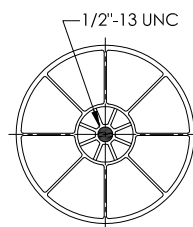
PLASTIC PISTON
