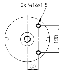
STEEL PISTON
