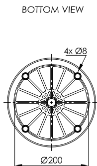
PLASTIC PISTON
