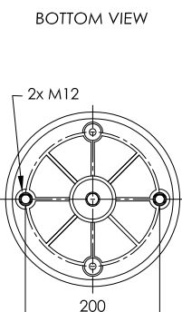
PLASTIC PISTON
