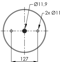
STEEL PISTON
