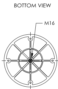
PLASTIC PISTON
