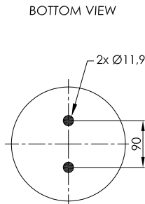
STEEL PISTON
