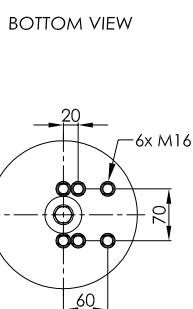
STEEL PISTON
