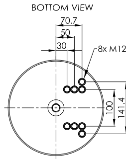
STEEL PISTON
