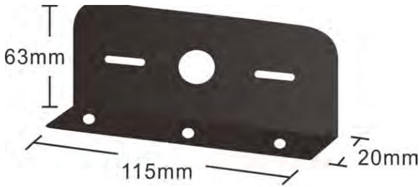
Bracket 7 Strobe mount
